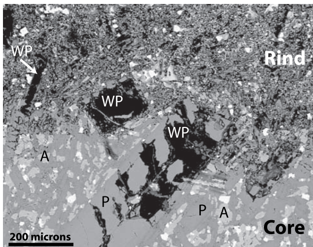
Figure 1. Scanning electron microscope backscatter image of one of the basalt clasts that electron microprobe data was collected for imaged across the reaction front. Labels are as follows: P, plagioclase; WP, weathered plagioclase; A, augite. Pores are black. There is a sharp contrast in porosity between the core and the rind as a result of dissolution of primary minerals. A large plagioclase crystal in the middle of the image is beginning to dissolve and create secondary porosity. Where other plagioclase crystals have dissolved, pores also remain.
