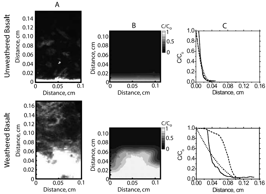
Figure 9. Comparison of results from diffusion experiments and models for (top) unweathered and (bottom) weathered basalt. (a) The \mu XRF image of Br concentrations measured at the surface of basalt samples in laboratory diffusion experiments after 7 days (see section 2.3). High Br concentrations near the y = 0 cm axis are white. (b) Contour plot of Br concentrations from 3-D diffusion simulations run for 7 days at the same scale as \mu XRF images. The position of the tracer front along the y axis in the models is similar to the position of the Br front in the laboratory diffusion experiments. (c) A plot of concentration of tracer relative to the original tracer concentration ( C/C_0 ) versus distance (cm) measured in laboratory diffusion experiments (solid line) and modeled in 1-D (dotted line) and 3-D (dashed line) numerical models.
