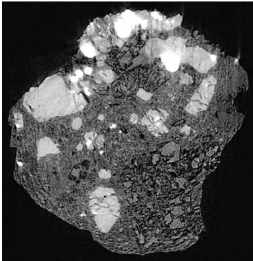
Figure 2. Two-dimensional image reconstructed from \mu CT data collected near the weathering interface of a weathering rind developed on a basalt clast from the 125 ka terrace. Dark areas are relatively less dense than light areas (black areas show porosity). All images rendered from the \mu CT data are provided in the auxiliary material. 1
