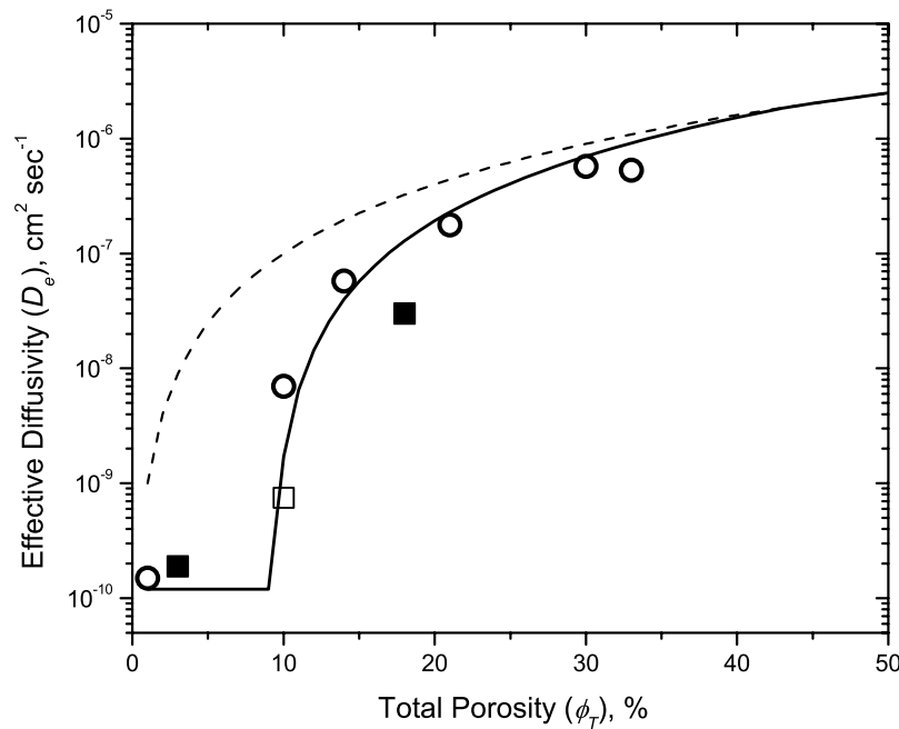
Figure 10. Values of D_e estimated from equation (3) using Archie's law with total porosity (dashed line) or from equation (8) using effective porosity as the scaling parameter (solid line). These estimates are compared with measured D_e in basalt (solid squares for diffusion experiments in this study and open squares for data from Sato et al. [1997]). Values of D_e calculated from numerical diffusion experiments are plotted as open circles. At porosities near and below the critical porosity, effective porosity is a better predictor of D_e than total porosity.
