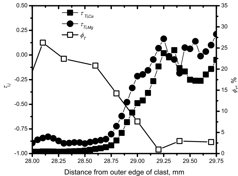
Figure 6. Values of \tau_{ij} for Ca and Mg and total porosity plotted versus distance from the outer edge of the basalt clasts from the 125 ka terrace. For clasts from the 125 ka terrace the weathering interface is generally located between 28.6 and 29.1 mm from the outer edge of the basalt clast. Here \tau_{ij} values for Ca and Mg decrease across the weathering front, consistent with weathering of plagioclase and augite. There is a corresponding increase in total porosity associated with weathering.
