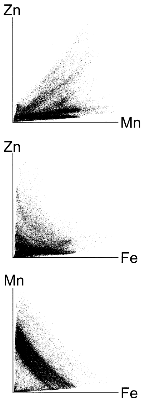
Fig. 2. Scatterplots for Zn, Mn, and \text{FeK}_\beta for the area shown in Figure 1. The scale limits for Zn, Mn, and Fe are 7, 250, and 50 arbitrary units, respectively.
