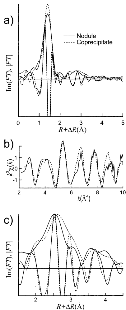
Fig. 12. Fourier transforms (FTs) of As EXAFS data in Figure 11. To make the higher shells more visible, we subtracted out a filtered first shell contribution from the k space data and redid the FT for sample and reference. The FTs for the data are shown in (a), the k space data with the first shells subtracted off are shown in (b), and the FTs of the subtracted data are shown in (c).
