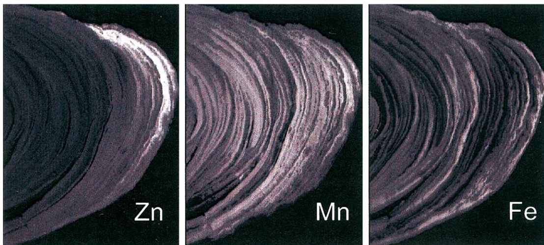
Fig. 1. XRF tricolor map of a ferromanganese nodule from the Baltic sea. Zn is coded as red, Mn as green, and Fe as blue. Separate monochrome maps for Zn, Mn and Fe are shown below the color maps. These maps are presented with positive contrast (bright=high concentration).
