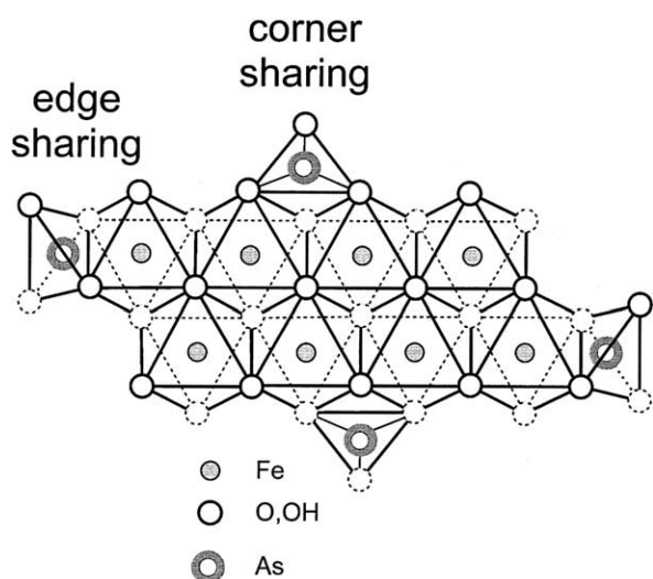
Fig. 13. Idealized structural units for As sorbed on 2-line ferrihydrite, after Manceau (1995). This diagram is meant to be qualitative only and not representative of the distances between \text{AsO}_4 tetrahedra. The O atoms shown in dotted lines are below the level of the Fe and As atoms.
