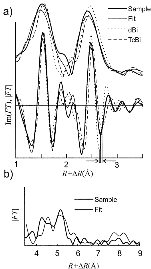
Fig. 7. Fourier transforms of Mn K-edge k^3\chi(k) EXAFS data in Figure 6. The magnitudes and imaginary parts are shown, with the magnitude shifted up for clarity. The curves are for the sample (heavy line), fit to dBi+TcBi (light line), dBi (dotted line), and TcBi (dashed line). It should be noted that small shifts in distance are more reliably detected by looking at the imaginary part than the magnitude. The upper panel shows the first two shells, and the lower shows the higher distances. Arrows point out the phase difference in the Fourier transform in the Mn-Mn region. The pure references and imaginary parts are omitted for clarity from the lower panel.
