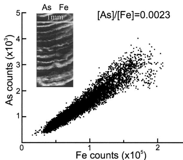
Fig. 3. Scatterplot for As and Fe in a section of the nodule. The inset shows a grayscale (positive-contrast) map in which the left side represents As and the right Fe.
