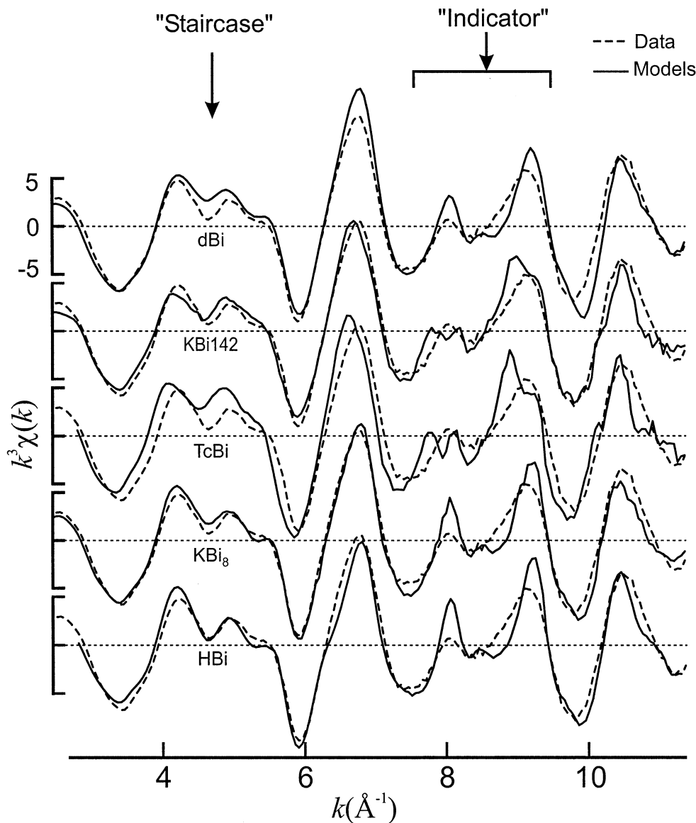
Fig. 6. Mn K-edge EXAFS for the sample (dashed lines) and five birnessite references (solid lines). Note the phase differences in the “staircase” region and the features in the “indicator” region. In this and the next two Figures, the EXAFS for the sample has been multiplied by 1.31 to compensate for overabsorption.
