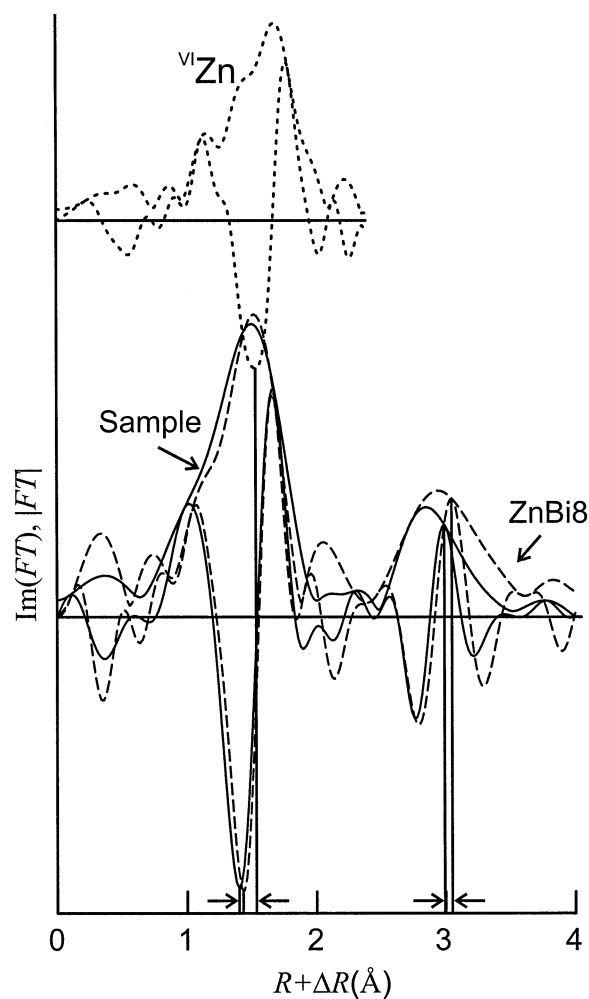
Fig. 10. Fourier transform of data for the sample and reference (solid, dashed) at the Zn K-edge. For comparison, the Zn-O shell of chalcophanite (all octahedral Zn) is shown in dotted lines. The positions of the minima in the imaginary parts are flagged to show the differences in Zn-O and Zn-Mn distances (arrows).
