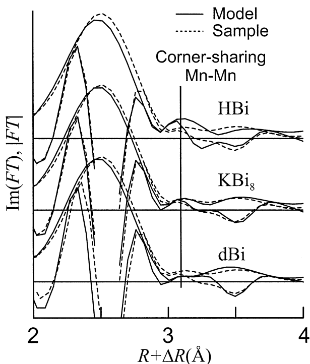
Fig. 8. Fourier transforms of Mn K-edge k^1\chi(k) . The data for the sample is in dashed lines, and the models in solid lines. The position of the corner-sharing (interlayer Mn) peak is indicated.
