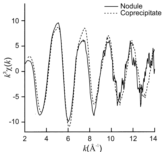
Fig. 11. As K-edge EXAFS from the sample (solid) and coprecipitate (As on ferrihydrite, dashed line).
